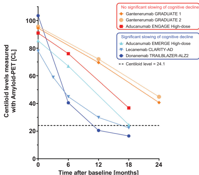
FIGURE 5 Amyloid- \beta removal profiles for Phase-III trials of aducanumab, donanemab, gantenerumab, and lecanemab as measured by Centiloid (CL). Sample sizes in the treatment arms varied for the individual trials and were at the last visit: N = 614 for donanemab, N = 210 for lecanemab, N = 50 (Graduate 1) and N = 41 (Graduate 2) for gantenerumab, and N = 109 (Emerge high-dose) and N = 112 (Engage high-dose) for aducanumab. Data points as reported in Sims et al. (2023), van Dyck et al. (2022), Bateman et al. (2023), and Budd Haeberlein et al. (2022). Placebo groups are not plotted and showed constant or slightly increasing amyloid levels over time, as expected. The dotted line represents 24.1 CL, the cutoff for amyloid-negativity as defined within the GRADUATE 1 and 2 trials and implemented in the head-to-head studies of donanemab versus Aduhelm.
