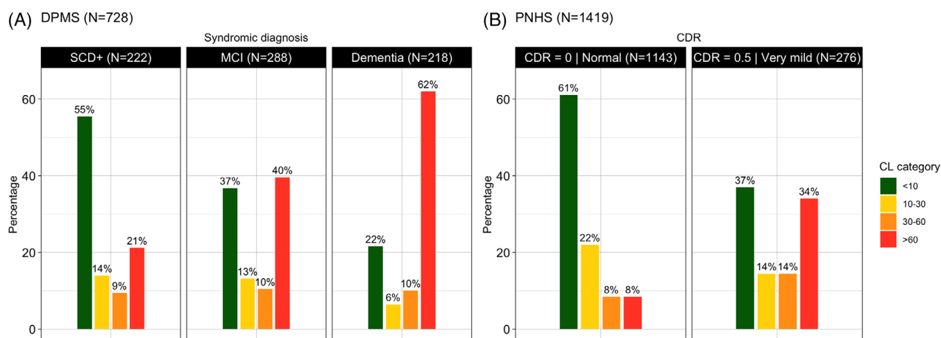
FIGURE 3 AMYPAD participants categorized by cognitive stage and baseline CL. Bar plots illustrate the distribution of CL groups across two studies, (A) DPMS and (B) PNHS, from the AMYPAD consortium. Subjects were categorized into four groups based on their baseline amyloid burden: <10 CL (no amyloid pathology), 10 to 30 CL (“intermediate range,” evolving amyloid pathology), 30 to 60 CL (established amyloid pathology with increased prevalence of tau positivity), and >60 CL (established amyloid pathology with high certainty of tau-PET positivity). AMYPAD DPMS and PNHS datasets are publicly available ( https://amypad.eu/data/ ). AMYPAD, Amyloid Imaging to Prevent Alzheimer’s Disease; CDR, Clinical Dementia Rating; CL, Centiloid; DPMS, Diagnostic and Patient Management Study; MCI, mild cognitive impairment; PNHS, Prognostic and Natural History Study; SCD+, subjective cognitive decline plus.
