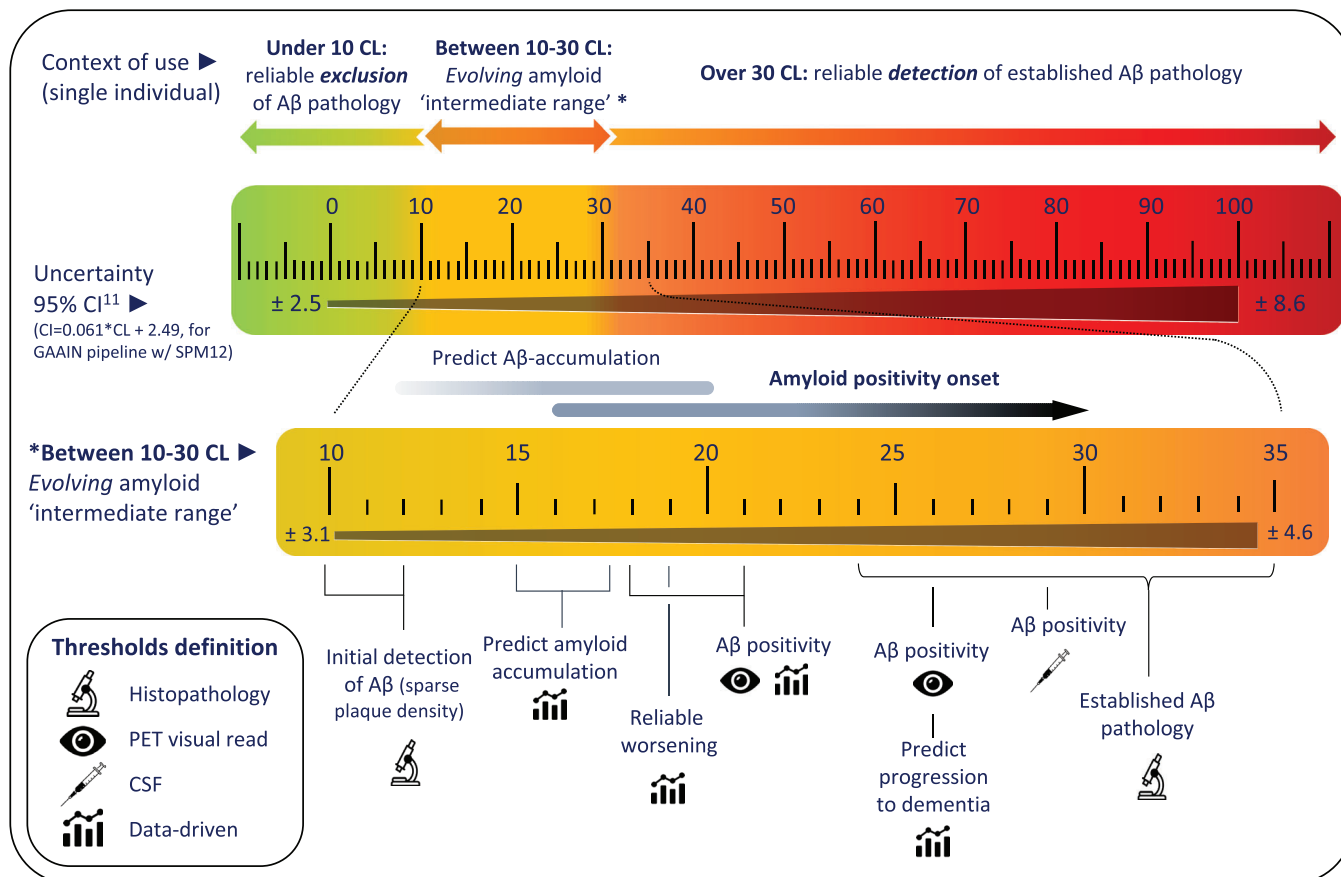
FIGURE 4 Overview of Centiloid scale interpretation. An illustrative figure summarizing the main studies regarding CL-based cut points to reliability exclude (<10 CL) and include (>30 CL) Aβ-pathology at the individual level. In addition, the 95% confidence interval across the scale is provided and detailed cutoffs in the "intermediate range" are highlighted. Aβ, amyloid-beta; CL, Centiloid; CI, confidence interval; CSF, cerebrospinal fluid; GAAIN, Global Alzheimer's Association Interactive Network; PET, positron emission tomography; SPM, Statistical Parametric Mapping.
